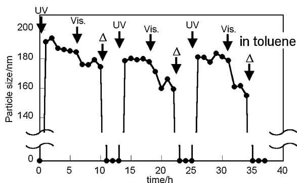
Figure 2. Particle size change of the supramolecule upon irradiation with UV and visible light in a toluene solution (20 °C, [2] = 3.0 \times 10^{-4} \text{ mol dm}^{-3} ).
